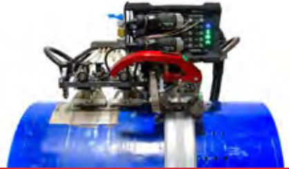
AUTOMATED GIRTH WELD INSPECTION SYSTEMS (PIPEWIZARD)
