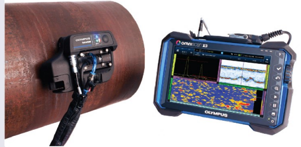
▶ CORROSION INSPECTION SCANNERS
